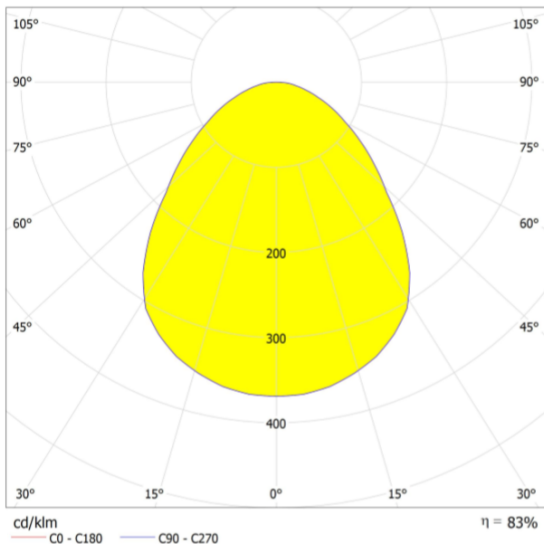
GDS Reality Series ALPCM 440mm Recessed 3000K 20W Microprism / LDC (Polar)
